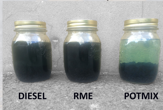
Test 2: Dissolution of hot mix asphalt after four hours.
