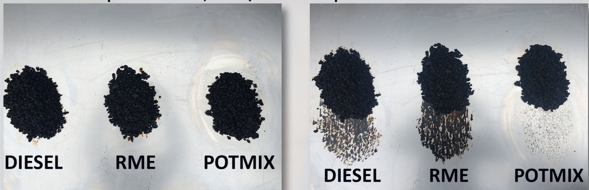
Test 1: Hot mix asphalt on diesel, FAME/RME and Asphalt Release. Result after five minutes.
